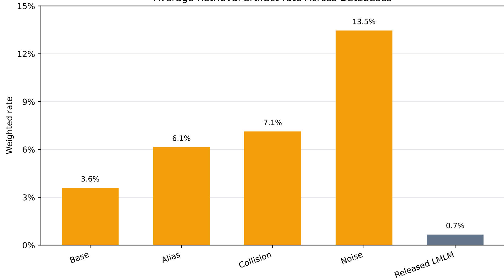
Average Retrieval artifact rate Across Databases
