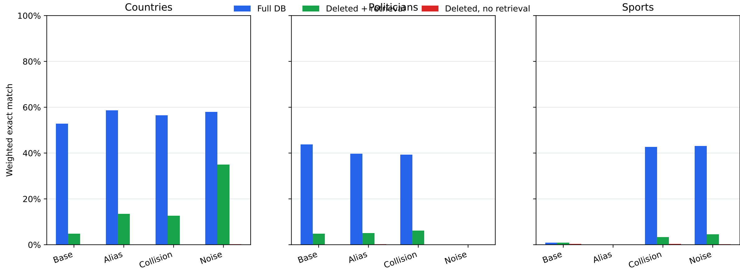
Exact Match by Domain, Database Variant, and State
