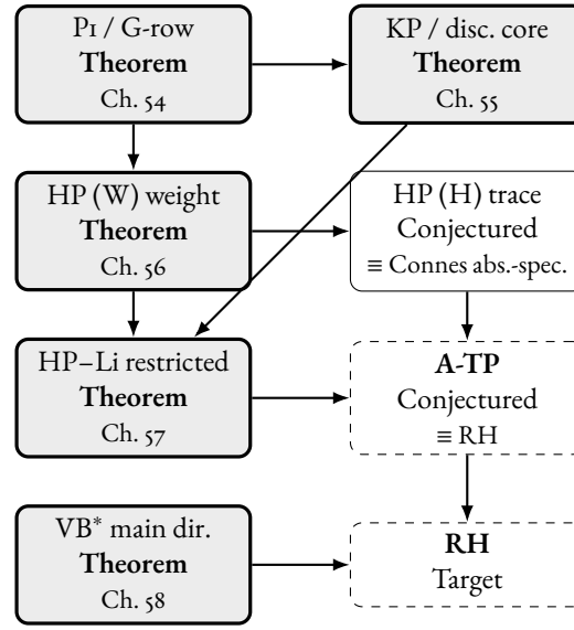
FIGURE 59.1: The refined minimal path to RH after Chapters 49–59. Shaded rounded boxes are unconditional theorems; the dashed rounded box is the single irreducible residual A-TP, strictly equivalent to RH. Ordinary rounded boxes are conditional intermediate statements. Each arrow is an implication established in the cited chapter.
