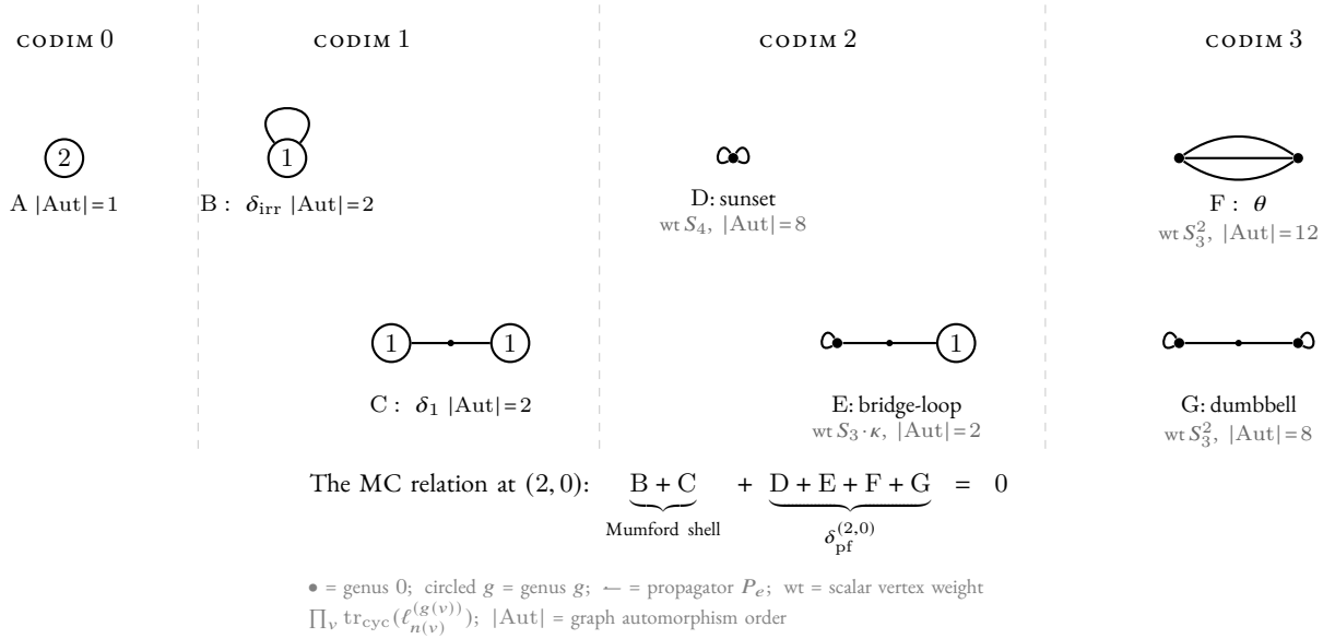
Figure 13.6: The MC tautological relation at (g, n) = (2, 0) as a graph sum. Each graph \Gamma contributes I_\Gamma \cdot w_\Gamma^{\text{cyc}} / |\text{Aut}(\Gamma)| where I_\Gamma is the Hodge integral on the boundary stratum and w_\Gamma^{\text{cyc}} is the scalar vertex weight. The sunset D has I_D = 0 . The planted-forest contributions from E, F, G combine to \delta_{\text{pf}}^{(2,0)} = S_3(10S_3 - \kappa)/48 , verified independently by pixon_shadow_bridge.py (82 tests).
