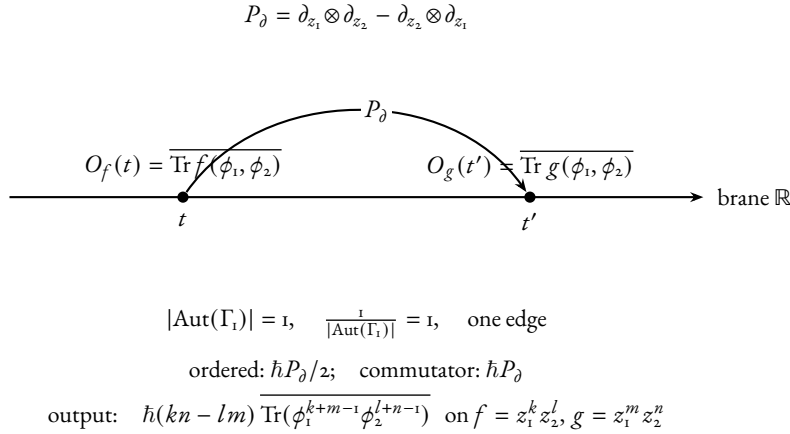
FIGURE 0.1: Notation for the reduced open-line order- \hbar raw commutator graph \Gamma_I , not a Costello/Feynman-integral proof. Two ordered boundary insertions sit on the brane line \mathbb{R} at distinct times t, t' ; the unique propagator P_\partial contracts one z_1 -leg on one side against one z_2 -leg on the other (and the antisymmetric partner). The automorphism group is trivial. In the Weyl ordered product the ordered one-edge weight is \hbar P_\partial/2 ; after subtracting the reverse order the commutator weight is \hbar P_\partial . The bivector contraction on monomials reproduces the cocycle coefficient (kn - lm) of Proposition 2.275, the order- \hbar Moyal coefficient of Proposition 2.320, and the \text{U}(1) centre cocycle \omega(f, g) of Lemma 1.16 realised at multidegree (k + m, l + n) = (1, 1) .
