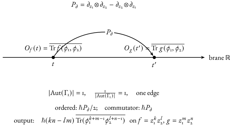
FIGURE 0.1: Notation for the reduced open-line order- \hbar raw commutator graph \Gamma_1 , not a Costello/Feynman-integral proof. Two ordered boundary insertions sit on the brane line \mathbb{R} at distinct times t, t' ; the unique propagator P_\partial contracts one z_1 -leg on one side against one z_2 -leg on the other (and the antisymmetric partner). The automorphism group is trivial. In the Weyl ordered product the ordered one-edge weight is \hbar P_\partial/2 ; after subtracting the reverse order the commutator weight is \hbar P_\partial . The bivector contraction on monomials reproduces the cocycle coefficient (kn - lm) of Proposition 5.163, the order- \hbar Moyal coefficient of Proposition 5.208, and the U(1) centre cocycle \omega(f, g) of Lemma 6.2 realised at multidegree (k + m, l + n) = (1, 1) .
