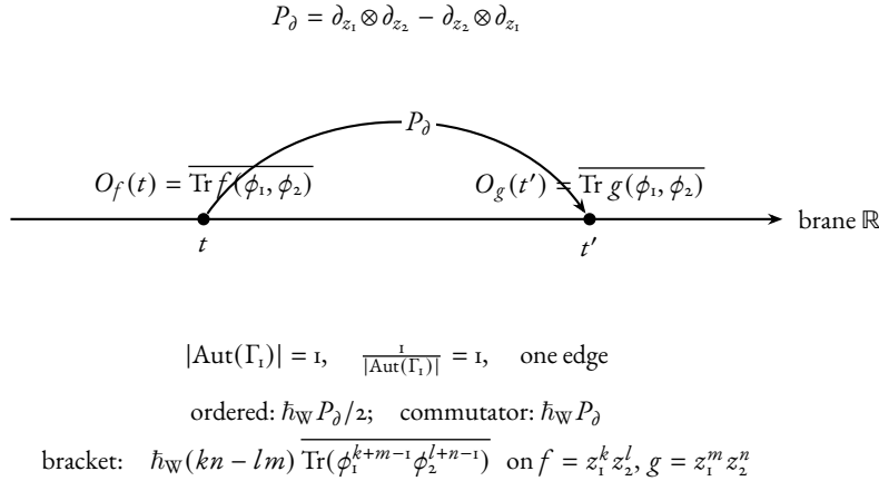
FIGURE 0.1: Notation diagram for the reduced open-line order- \hbar_W raw commutator graph \Gamma_1 . Two ordered boundary insertions sit on the brane line \mathbb{R} at distinct times t, t' ; the single boundary propagator P_\partial contracts one z_1 -leg on one side against one z_2 -leg on the other (and the antisymmetric partner). The automorphism group is trivial. In the Weyl ordered product the ordered one-edge weight is \hbar_W P_\partial / 2 ; after subtracting the reverse order the commutator weight is \hbar_W P_\partial . The bivector contraction on monomials reproduces the cocycle coefficient (kn - lm) of Proposition 5.175, the order- \hbar_W Moyal coefficient of Proposition 5.220, and the \text{U}(1) centre cocycle \omega(f, g) of Lemma 6.2 realised at multidegree (k + m, l + n) = (1, 1) .
