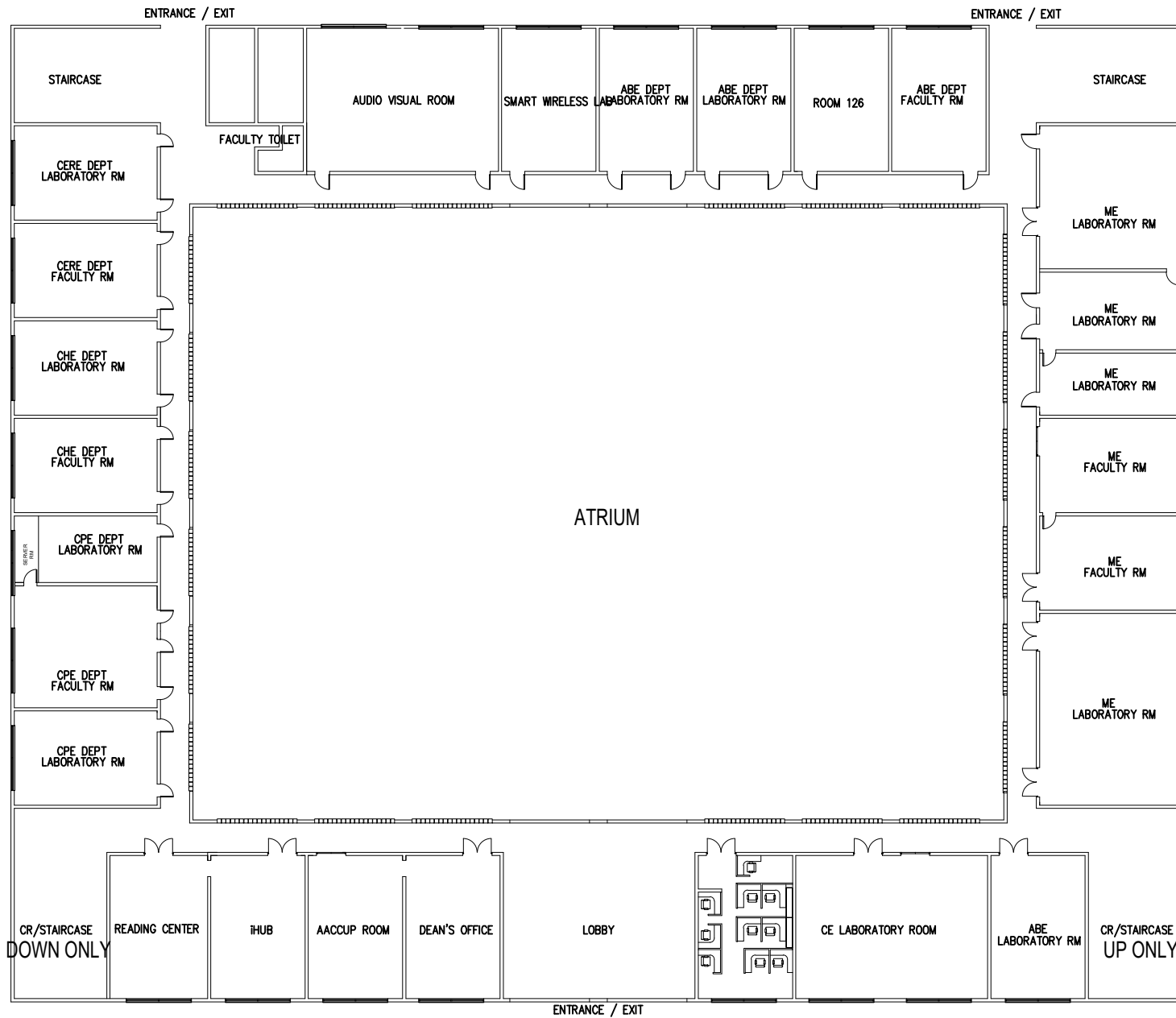
COE BUILDING – GROUND FLOOR
