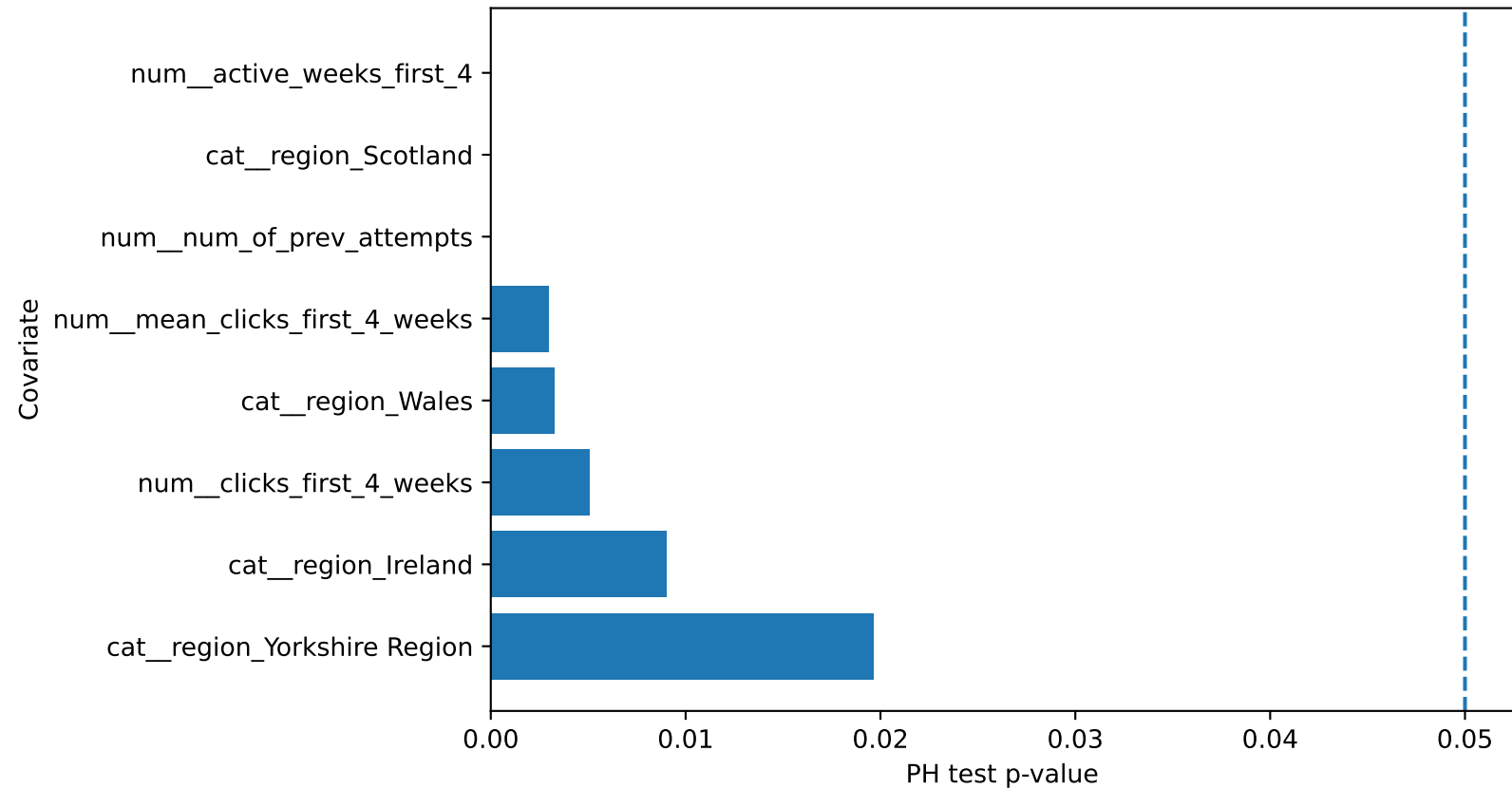
Comparable Cox PH diagnostic (smallest p-values)
