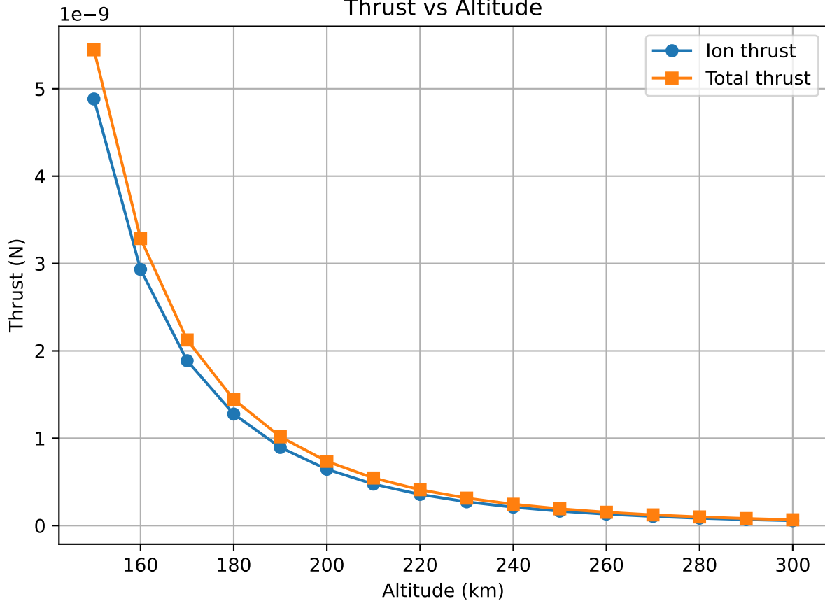
Thrust vs Altitude
