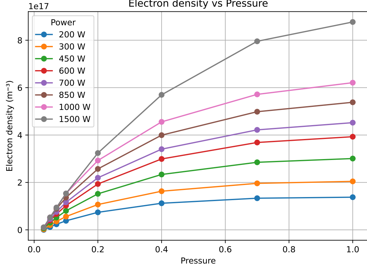
Electron density vs Pressure
