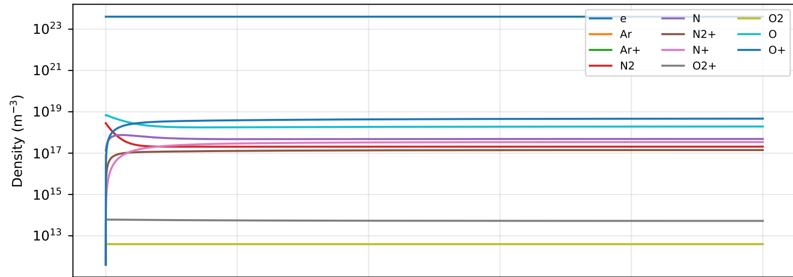
E09 Species Concentrations Over Time at 250 km
