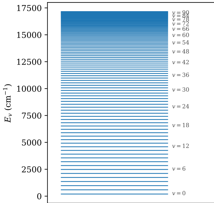
Vibrational levels (J=0)
