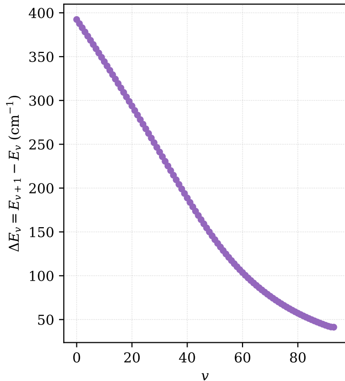
Level spacing (anharmonic roll-off)
