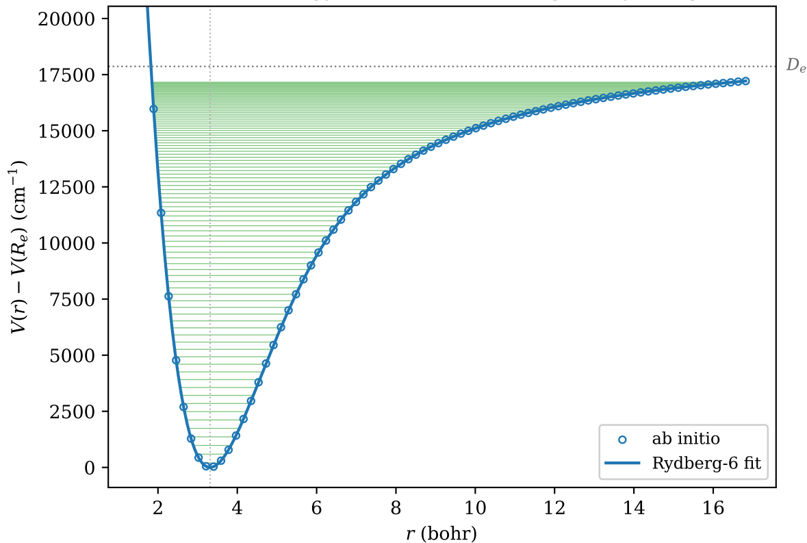
Potential energy curve and sixth-degree Rydberg fit
