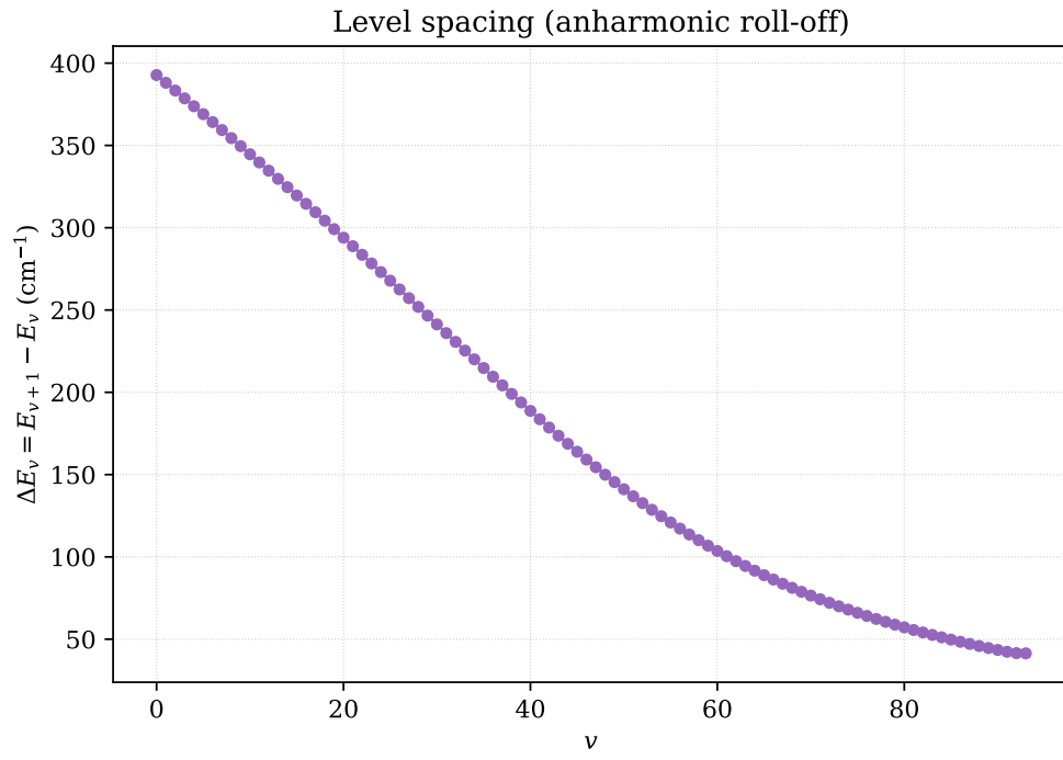
Figure 4: Anharmonic decrease of the level spacing \Delta E_v = E_{v+1} - E_v with v , up to dissociation.
