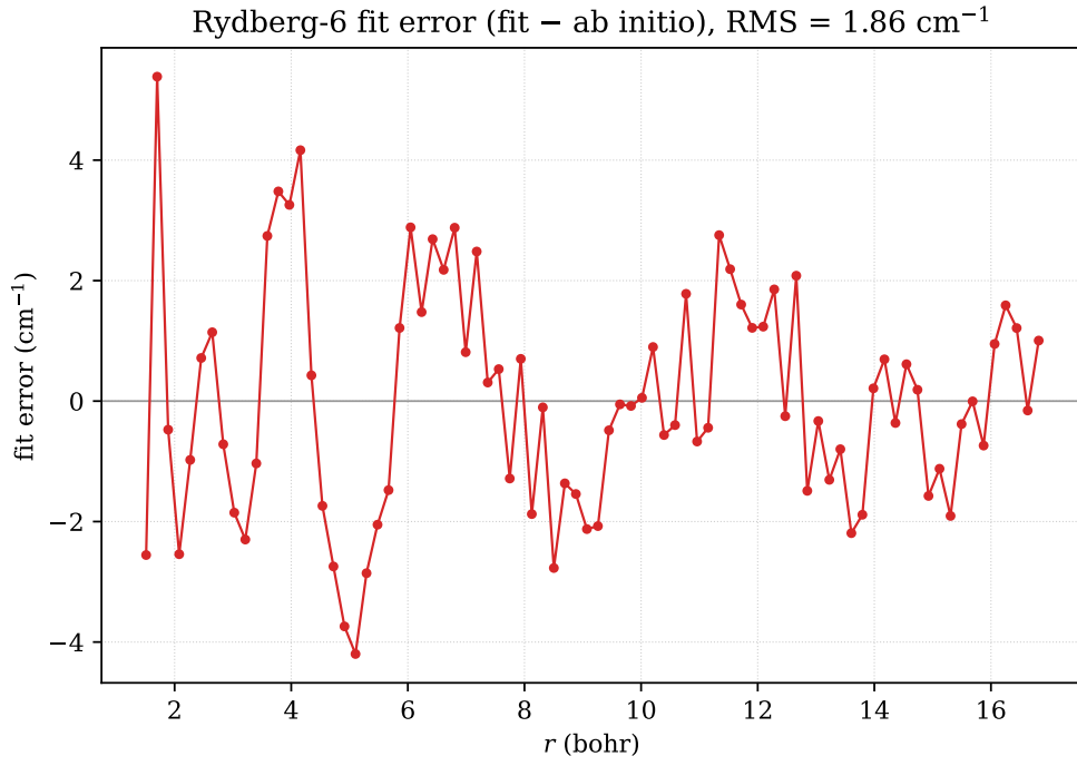
Figure 2: Residual of the sixth-degree Rydberg fit, fit – ab initio, over the whole grid.
