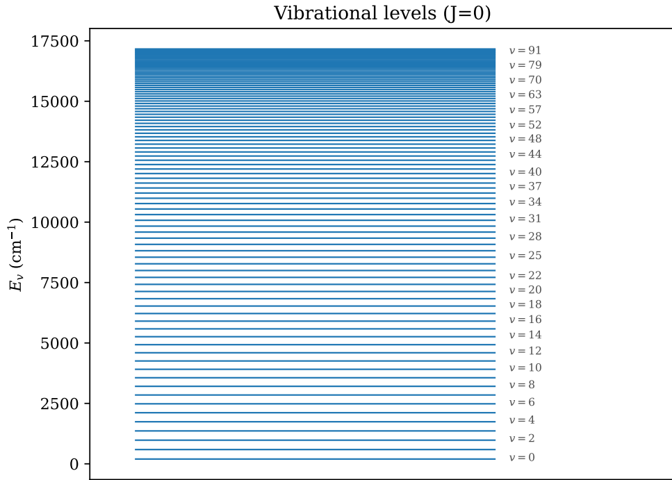
Figure 3: Vibrational energy-level ladder of the J=0 run: every bound state below D_e , labelled where the spacing allows.
