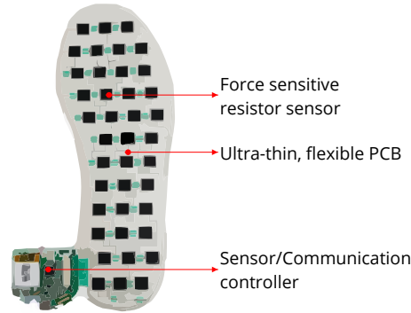
Fig. 2. The PediSol Smart Insole used in the XRGait system. This is an insole inserted into the user's shoe with a grid of pressure sensors to track how the user balances their weight during gait training.
