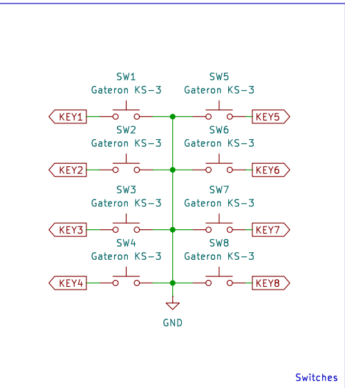
Switches
