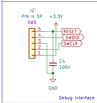
Debug Interface
