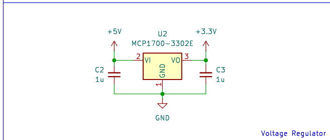
Voltage Regulator
