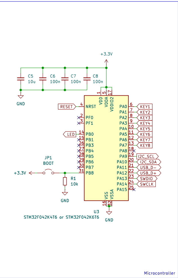
Microcontroller
