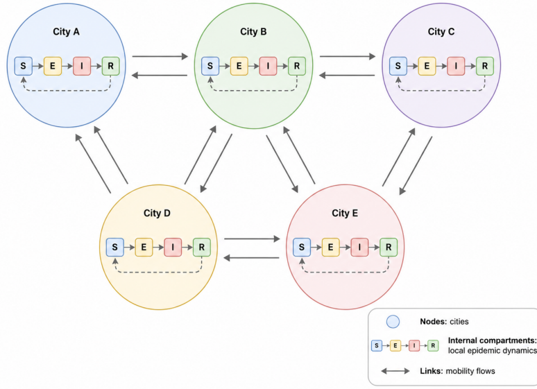
Figure 1: Metapopulation epidemic framework. Each circle represents a city, modelled as a local subpopulation with its own compartmental epidemic dynamics. The internal compartments illustrate a generic SEIR-type progression: S denotes susceptible individuals, E exposed individuals who are infected but not yet infectious, I infectious individuals, and R recovered or removed individuals. The dashed return arrow indicates that some models, such as SIS or SEIRS, allow individuals to become susceptible again. Arrows between cities represent mobility flows that can transport susceptible, exposed, or infected individuals and seed outbreaks elsewhere. Inspired by metapopulation epidemic models such as Colizza and Vespignani [16].
