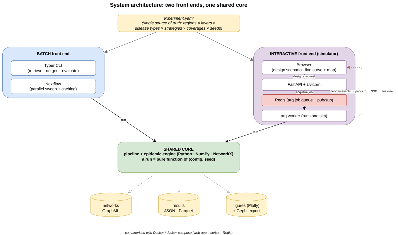
Figure 14: System architecture: one shared engine behind the interactive simulator and the programmatic runs, writing to a common results pipeline.
