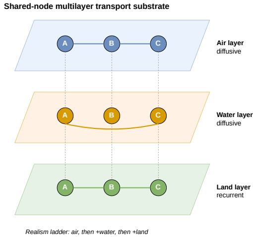
Figure 4: Shared-node multilayer substrate. Each city is one shared node present on every layer it uses (vertical dashed links); solid links are routes on that layer, drawn only where a route exists (not all-to-all). Air and water couple cities by diffusive relocation, land by recurrent commuting; the realism ladder adds water, then land.
