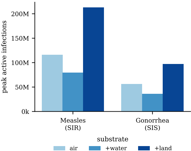
Europe: peak outbreak by disease and realism
