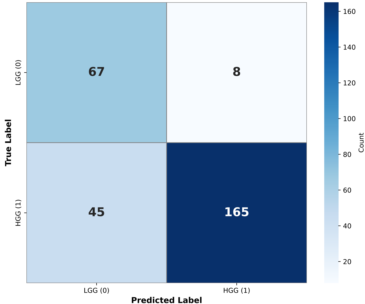
Confusion Matrix: Baseline Ensemble (Threshold = 0.41) TN=67, FP=8, FN=45, TP=165
