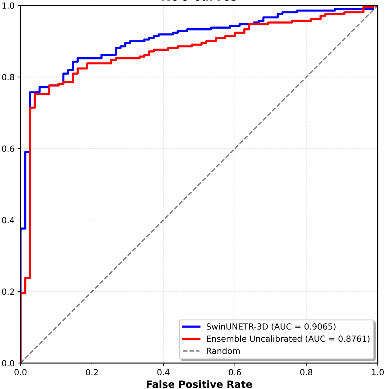
ROC Curves
