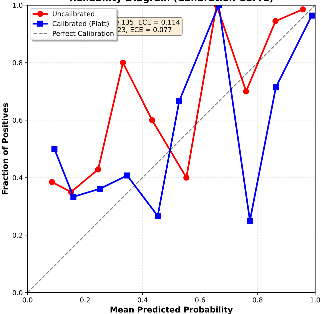
Reliability Diagram (Calibration Curve)
