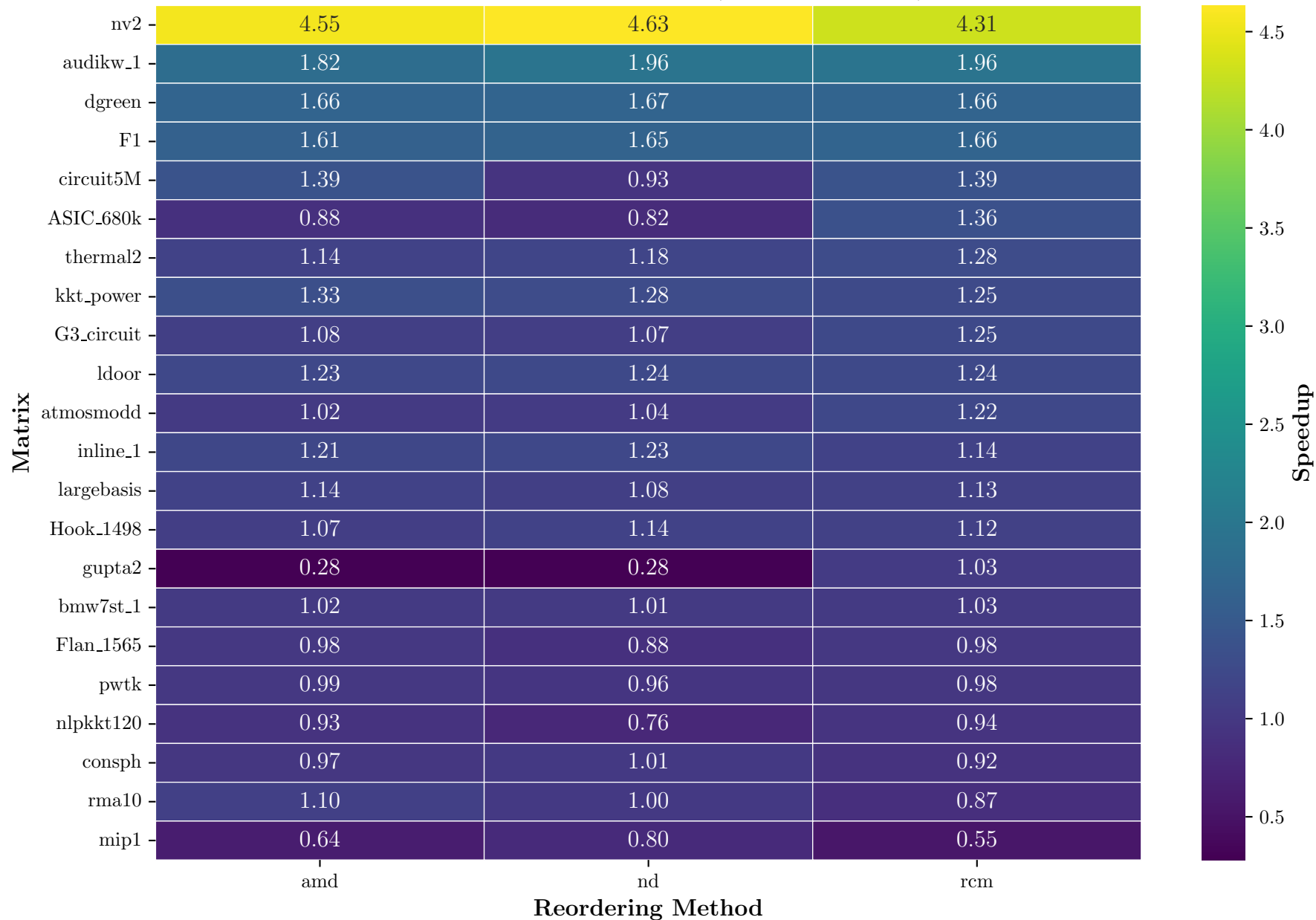
Speedup per Reordering (4 threads, x86)
