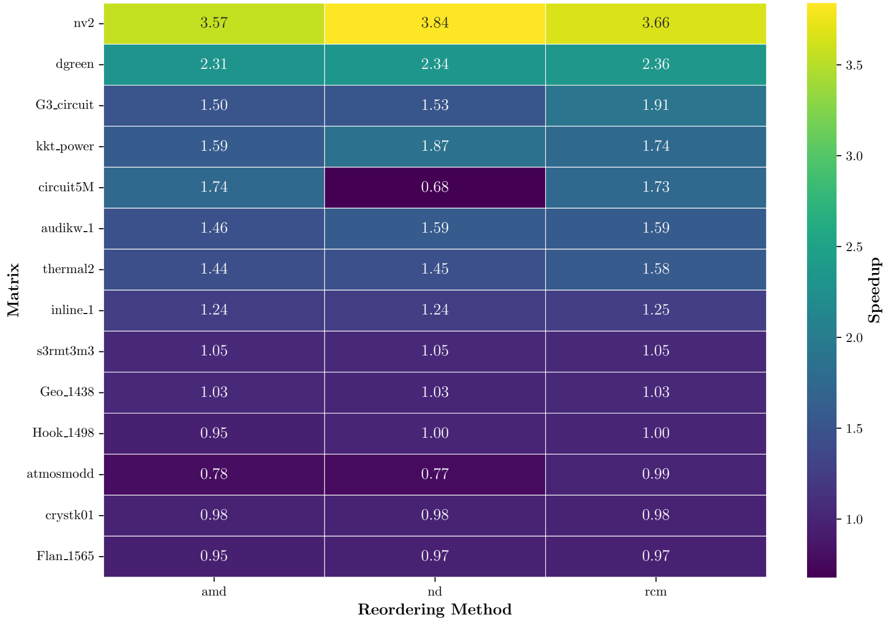
Speedup per Reordering (4 threads, ARM)
