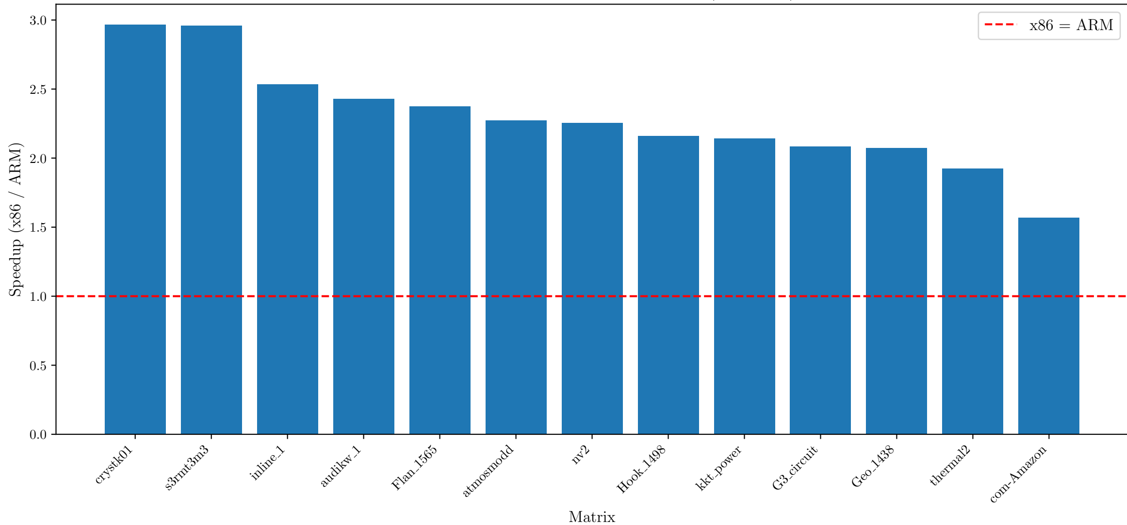
Performance Comparison: x86 vs ARM (4 threads)
