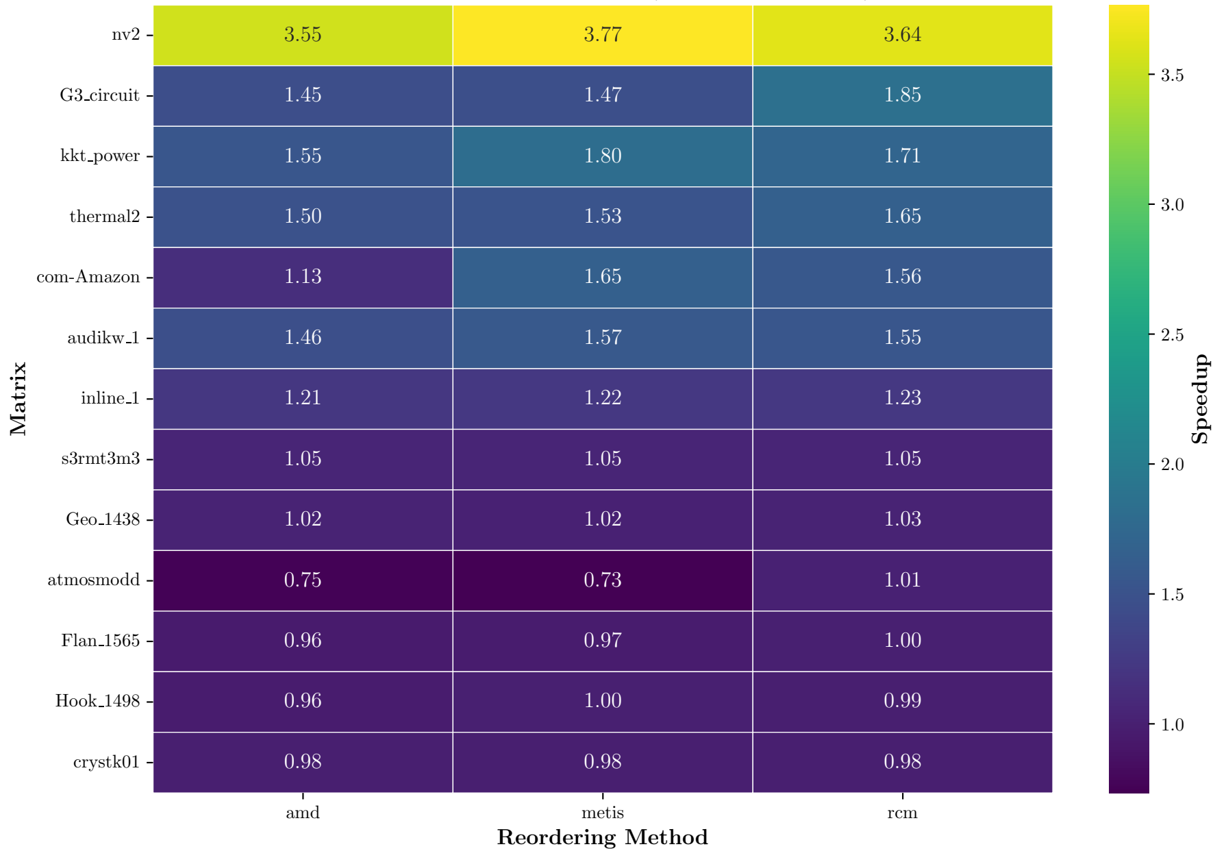
Speedup per Reordering (4 threads, ARM)
