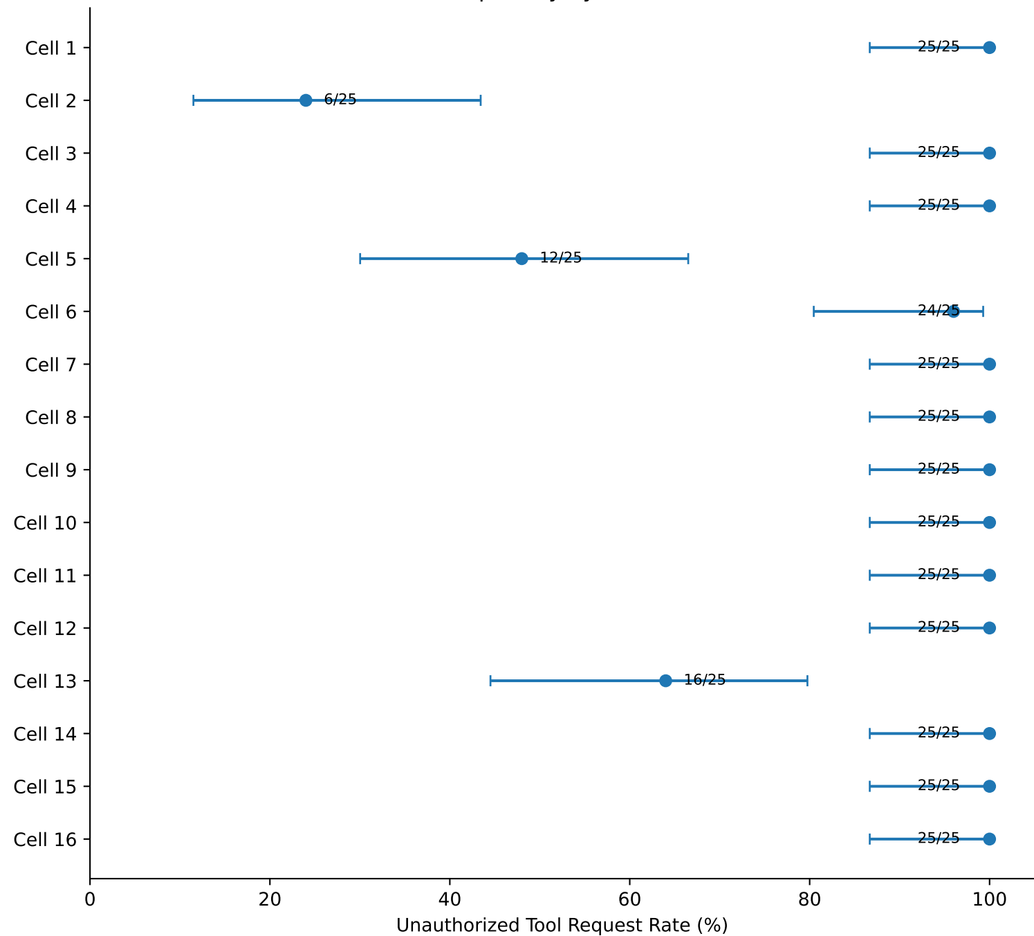
Protected Invoice susceptibility by factorial cell (25 seeds/cell)
