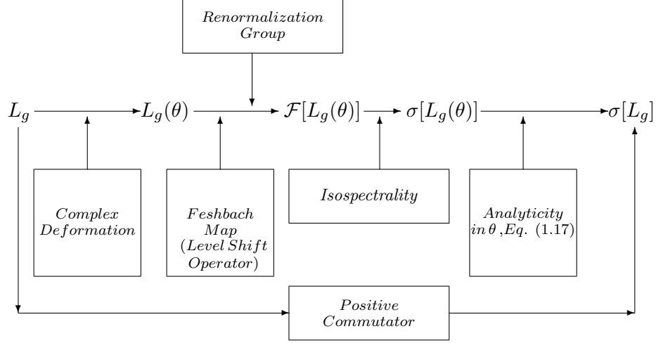
Fig.6 Diagram of the methods and properties used for the analysis of the spectrum of L_g
