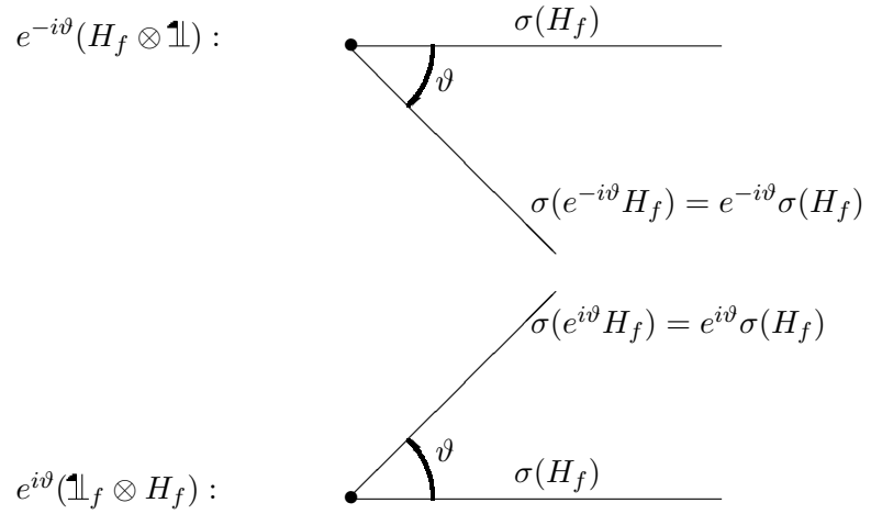
Fig.9 Rotation of the spectrum of H_f . Top: rotated by an angle of -\vartheta . Bottom: rotated by an angle of \vartheta
