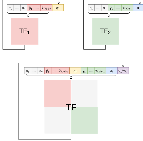
Fig. 3.4: Visual representation of the construction for disjunction
