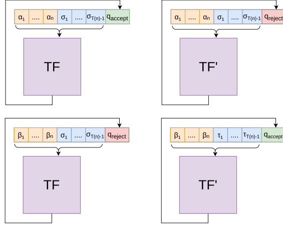
Fig. 3.3: Visual representation of the construction for complement
