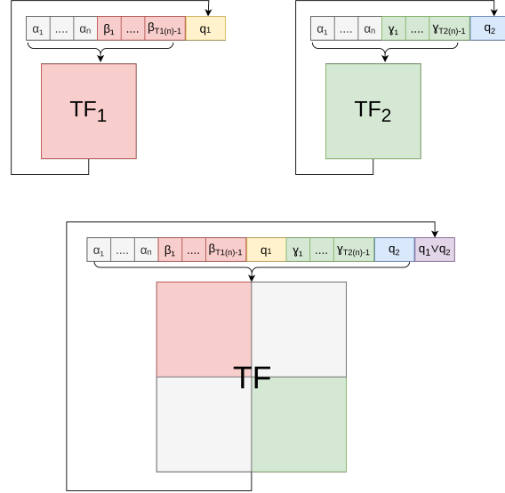
Fig. 3.5: Visual representation of the construction for disjunction
