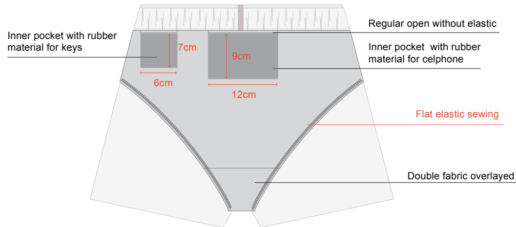
Inside body: Polyamide spandex fabric knit
