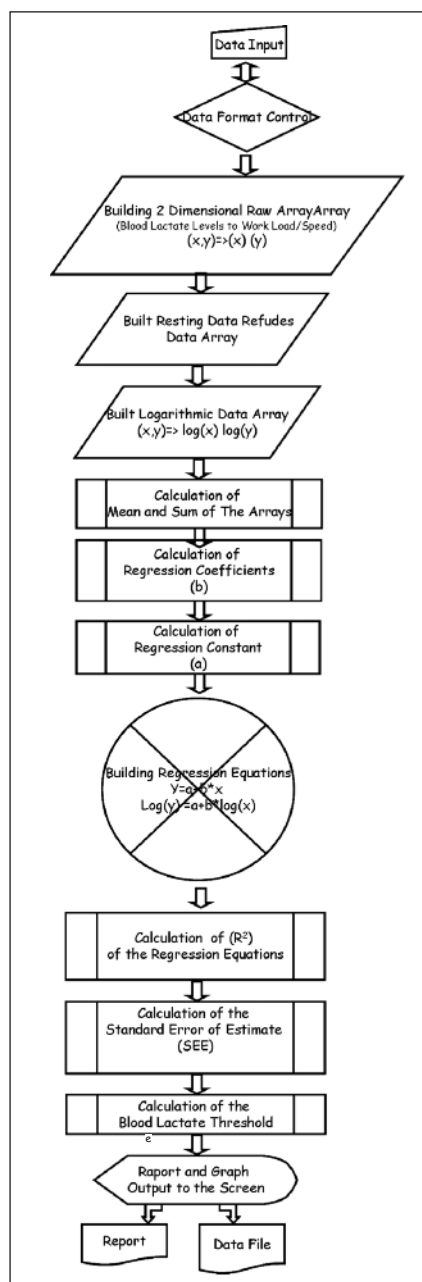
FIGURE 3: Algorithm of the software.
