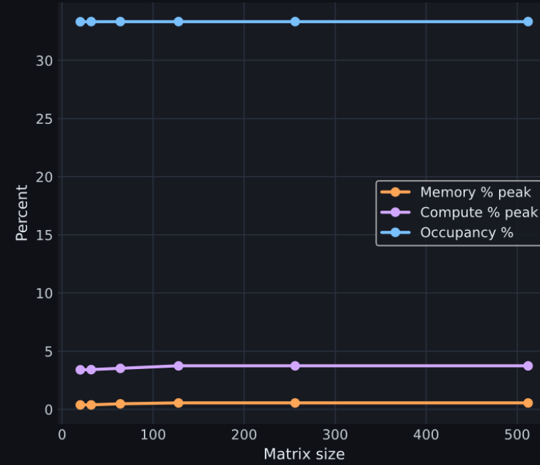
Profiler metrics vs size
