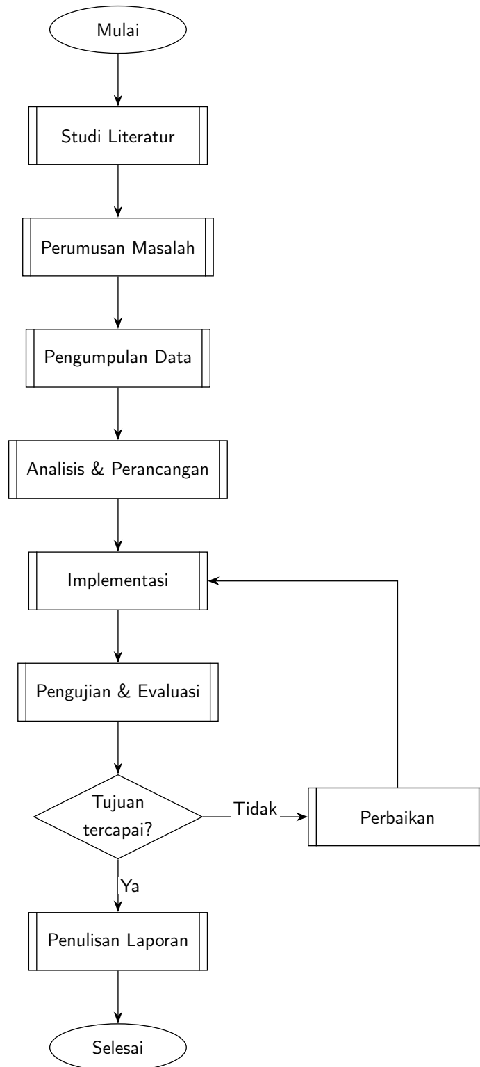
Gambar 3.1: Alur penelitian
