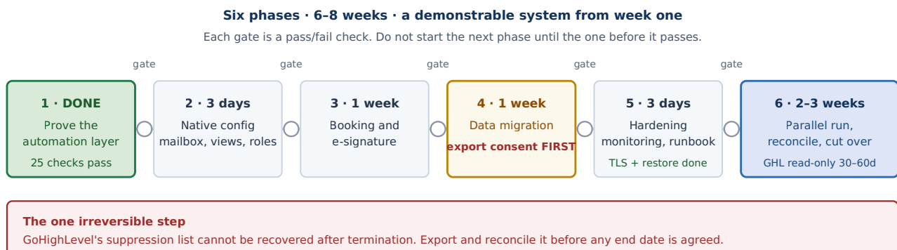
Figure 4 · Delivery sequence. Phase 1 is complete and two Phase 5 items — TLS behind a reverse proxy, and a restore-tested backup — are already done. The gates matter more than the durations: a phase that starts before the previous one passes moves the failure later, where it costs more.
