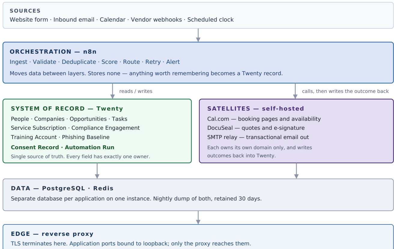
Figure 1 · The four layers. The load-bearing rule is that n8n stores nothing: if a fact matters, it lives in Twenty, which is what makes any single component replaceable without losing history.
