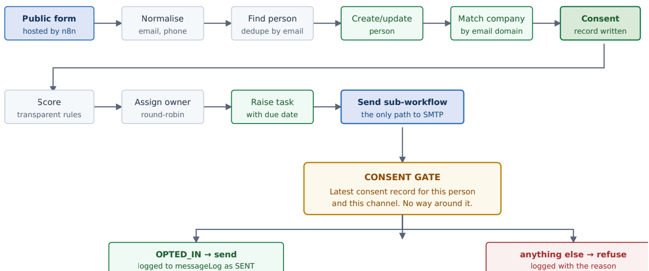
Figure 2 · Lead capture, end to end. The consent gate sits inside the send sub-workflow rather than in each calling workflow — a workflow author cannot forget it, because they never touch SMTP directly. Both outcomes are written to the CRM, so a refusal is evidence rather than silence.
