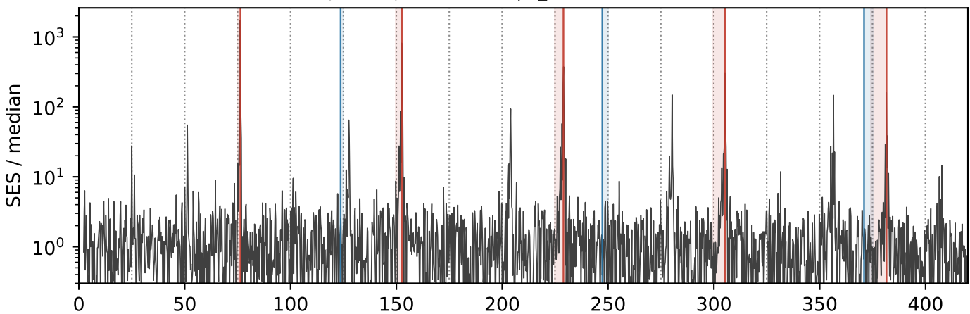
(c) CWRU 130, 6205, cepstrum pre-whitened | f_r = 29.93 Hz
