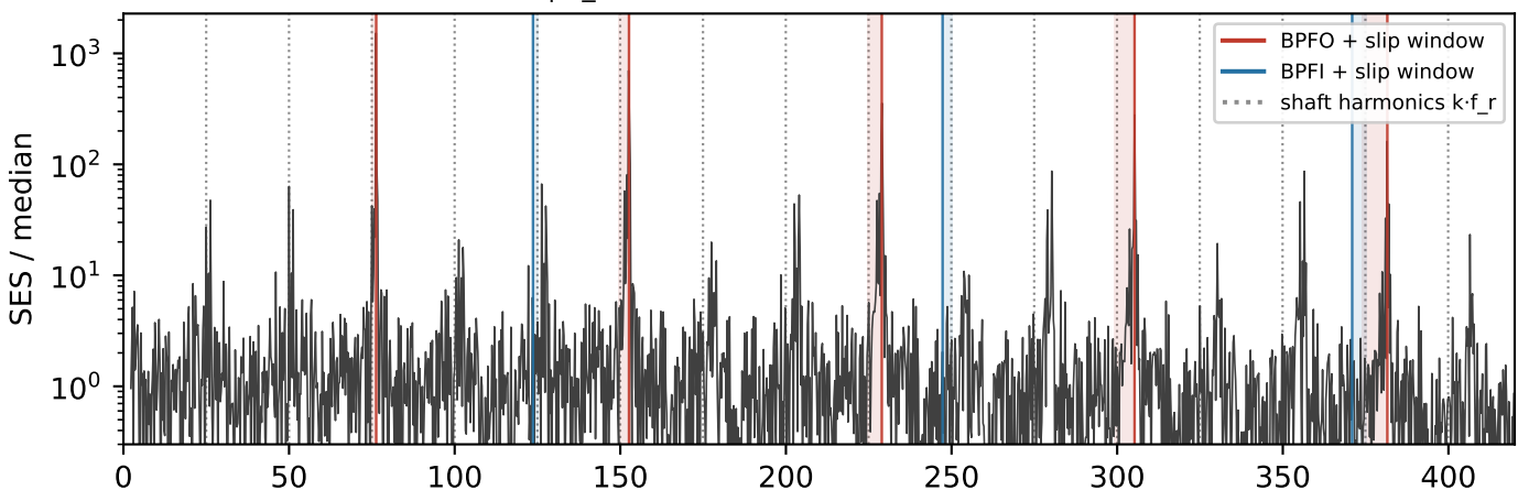
(b) Paderborn KA04, 6203, cepstrum pre-whitened | f_r = 24.99 Hz, band 8-11 kHz
