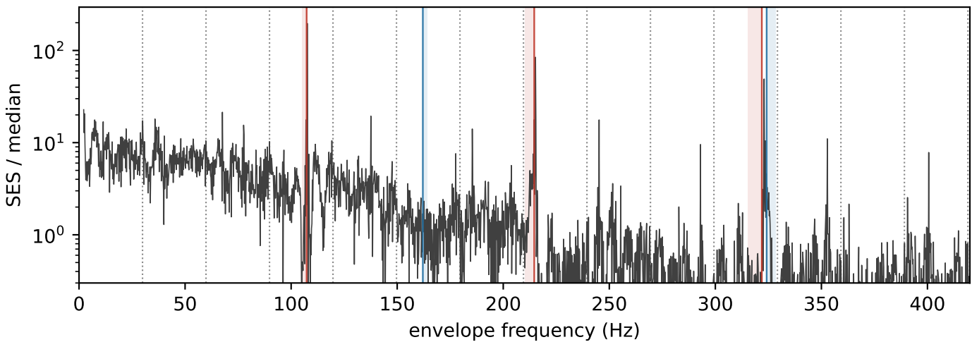
(c) CWRU 130, 6205, cepstrum pre-whitened | f_r = 29.93 Hz
