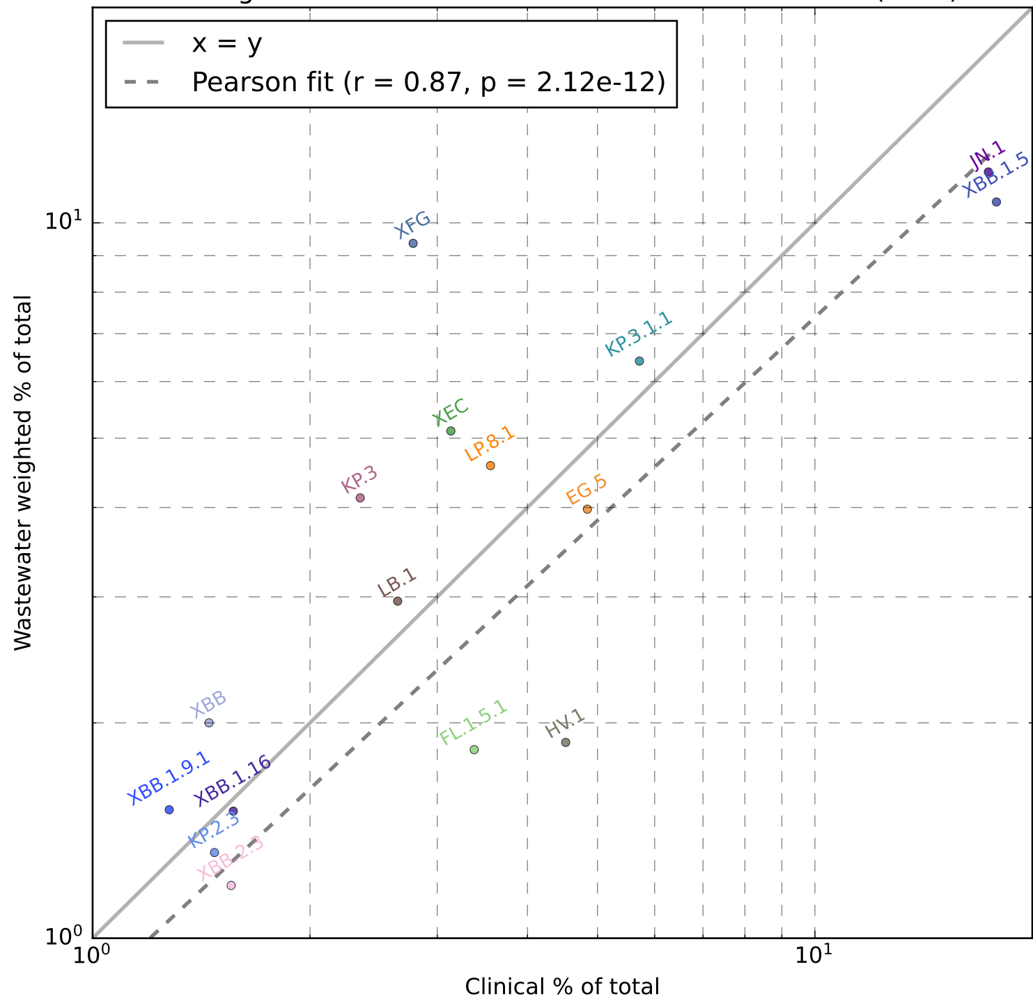
Lineage Relative Abundance: Clinical vs Wastewater ( \geq 1\% )
