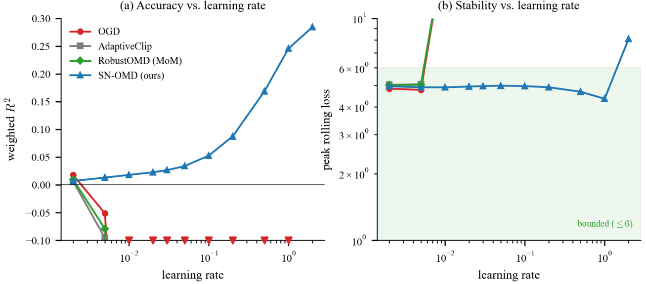
Figure 3. Main result (continuous multi-regime stream, causal standardization, per-row). (a) Weighted R^2 vs. learning rate: SN-OMD climbs monotonically to \approx 0.28 and never diverges, while OGD and both clippers cliff above \text{lr} = 10^{-2} (off-scale markers). (b) Peak rolling loss: SN-OMD stays bounded ( \approx 5 ) everywhere; the others explode.
