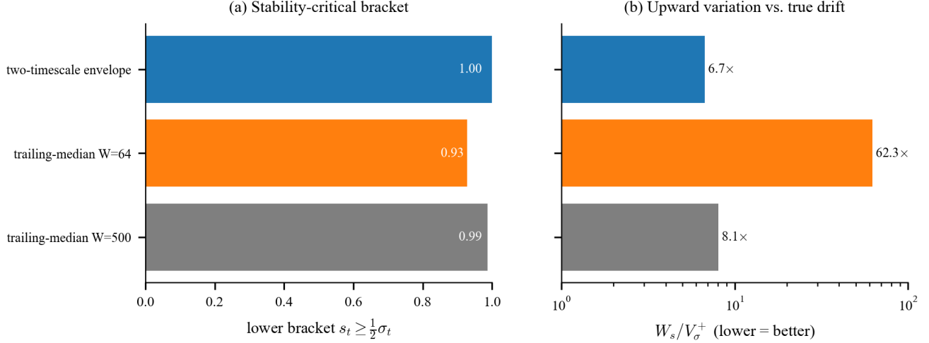
Figure 5. Discharging Assumption 3.2. A two-timescale “peak-hold” scale tracker on the real gradient-scale process (a) holds the stability-critical lower bracket s_t \geq \frac{1}{2}\sigma_t at every round, while (b) attaining the smallest upward variation W_s/V_\sigma^+ . A fast trailing median tracks the scale but churns (62×); a slow one is smooth but lags regime onsets and violates the lower bracket.
