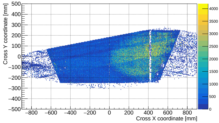
Figure 6: Cross Y vs X distribution. Events are weighted by E_U .
