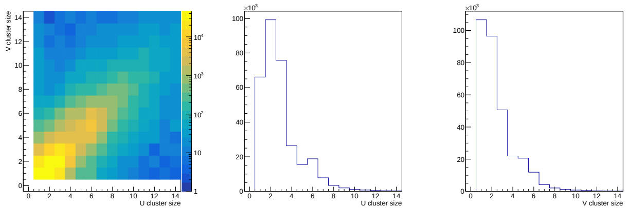
Figure 13: Cluster size distributions: Left: "V vs U" cluster sizes, middle: U cluster size, and the right is the V cluster.
