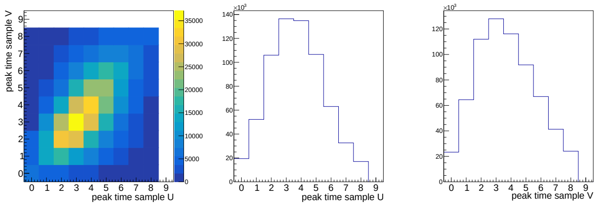
Figure 10: Peak time distributions: Left: "V vs U" cluster peak time, middle: U cluster peak time, and the right is the V cluster peak time.
