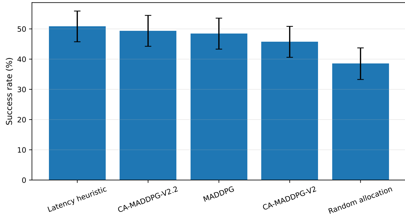
Fixed 100-Episode Performance Comparison
