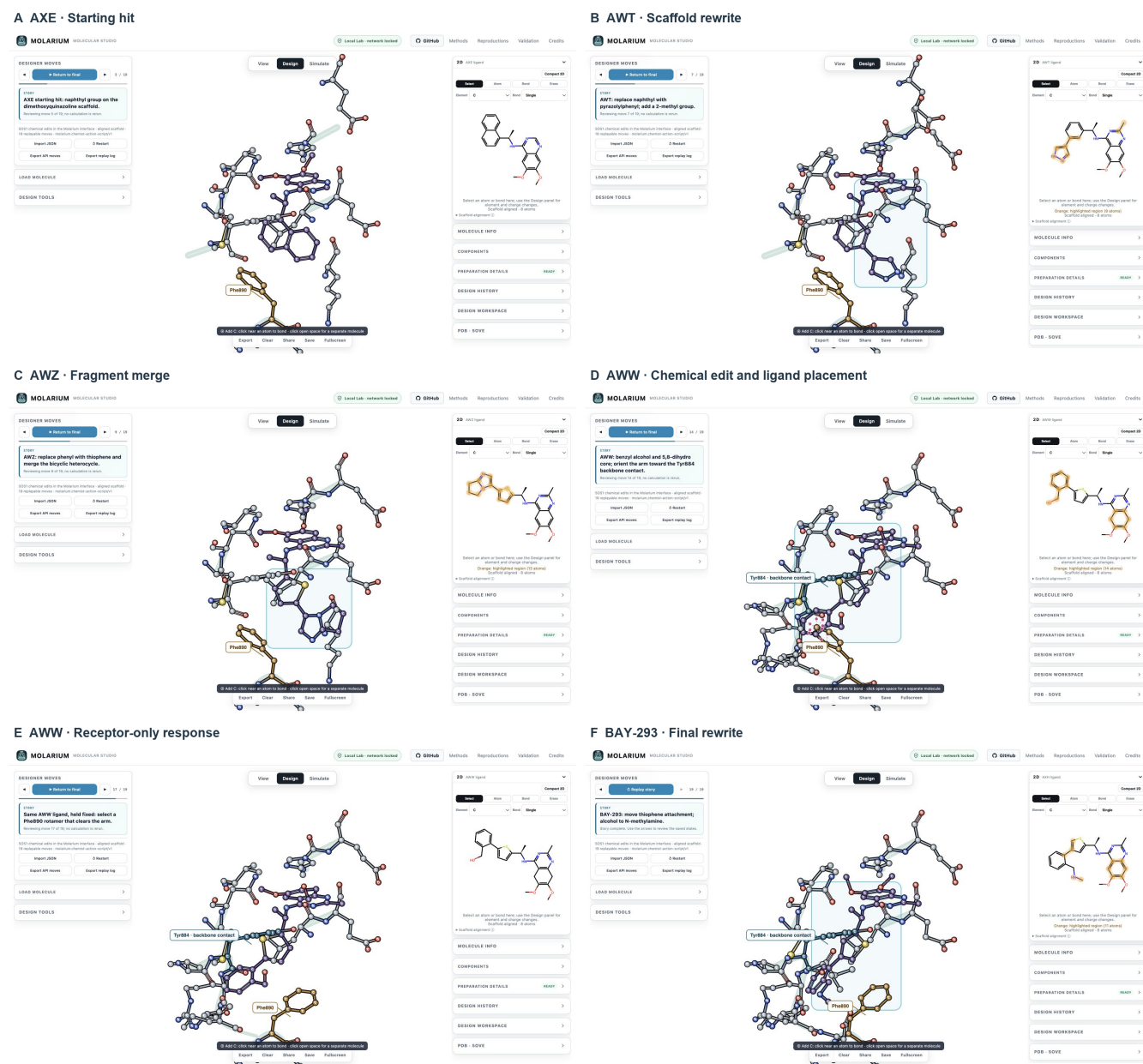
Figure 3: Agent-directed replay of the design trajectory of SOS1 inhibitor BAY-293 [30]. (A) AXE starting hit. (B) AWT: replace naphthyl with pyrazolylphenyl and add a 2-methyl group. (C) AWZ: replace with thiophene and a bicyclic heterocycle. (D) AWW: swap heterocycle for benzyl alcohol, then orient the arm toward the Tyr884 backbone-carbonyl contact. (E) Hold the same AWW ligand fixed while selecting a Phe890 rotamer that clears the arm. (F) BAY-293: move the thiophene attachment and replace the alcohol with an N-methylamine. Orange 2D highlights mark added atoms and local chemical changes relative to the preceding structure. The crystal series informed the design hypothesis, but later crystal coordinates were not used to generate these states.
