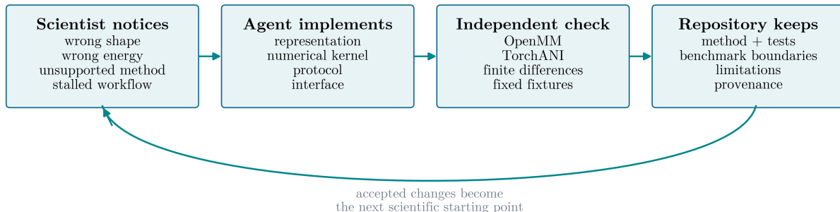
Figure 4: The scientist-agent build loop. Scientific needs and objections are translated into software changes, while each new capability is paired with claim-defining tests, reference evidence, applicability limits, and provenance. The ability to generate a workflow and the ability to specify how its claim could fail are treated as parts of the same scientific result.
