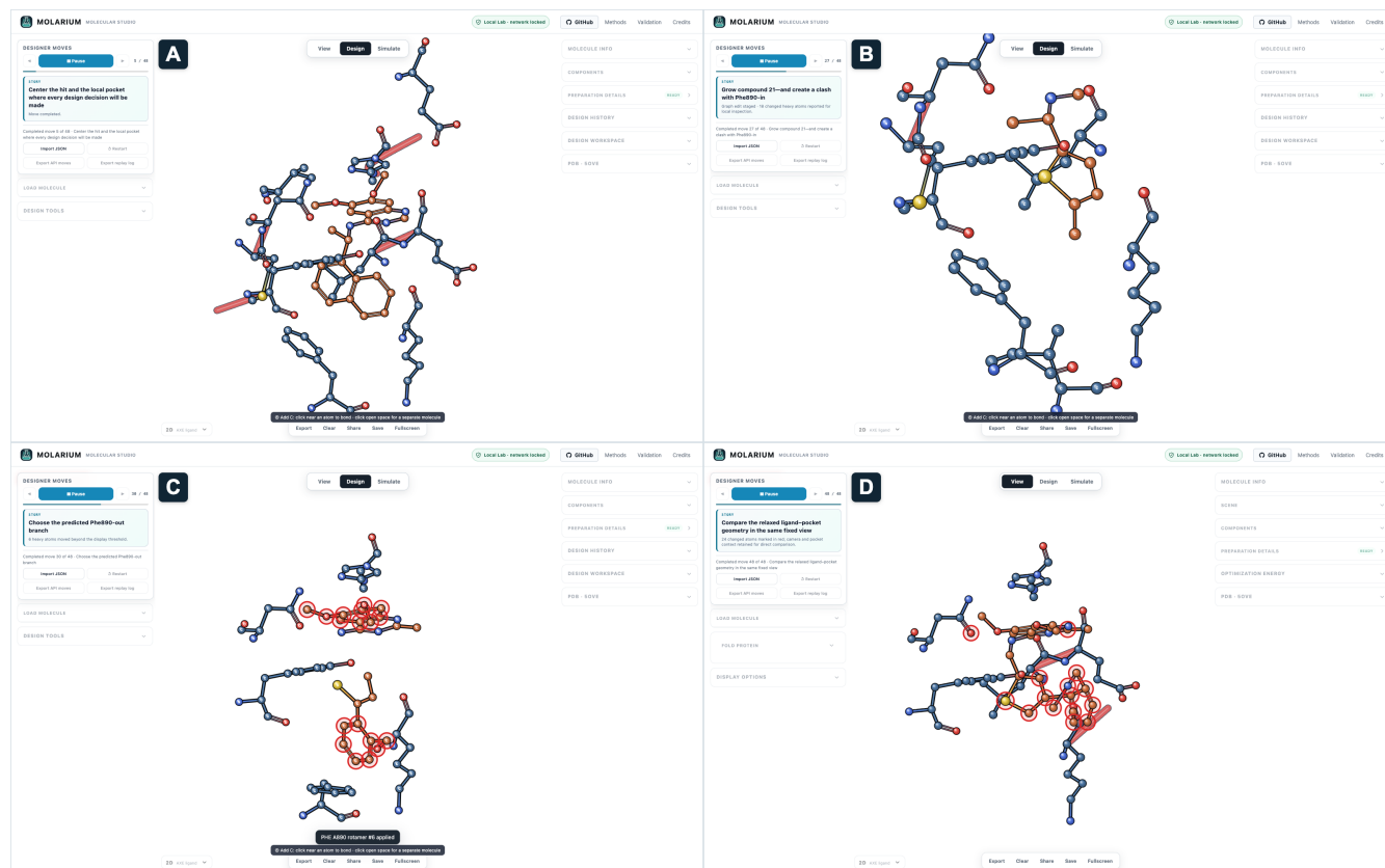
Figure 2: Hit-only SOS1 design replayed in the Molarium interface through the public Chemist Actions API. (A) The prepared 5OVE/AXE hit and local pocket are centered before prospective design; this was the sole coordinate-bearing input. (B) Sequential scaffold rewriting and growth produces compound 21 in the Phe890-in volume, and the visible replay caption records the resulting clash. (C) Side-chain enumeration selects the predicted Phe890-out branch; the interface reports PHE A890 rotamer 6 and marks the affected atoms for review. (D) The final BAY-293 ligand-pocket state is inspected after coupled WebGPU relaxation in the same fixed view. Red rings in panels C and D are interface change markers, not duplicate molecules. The interface replay ends at this prediction and does not open 5OVI. Independent post-freeze comparison with 5OVI subsequently gave a receptor-aligned, graph-symmetry-minimized ligand RMSD of 1.215 Å and Phe890 \chi_1 values of -172.43^\circ in the prediction and -166.55^\circ in the crystal; those validation coordinates did not seed the replay.
