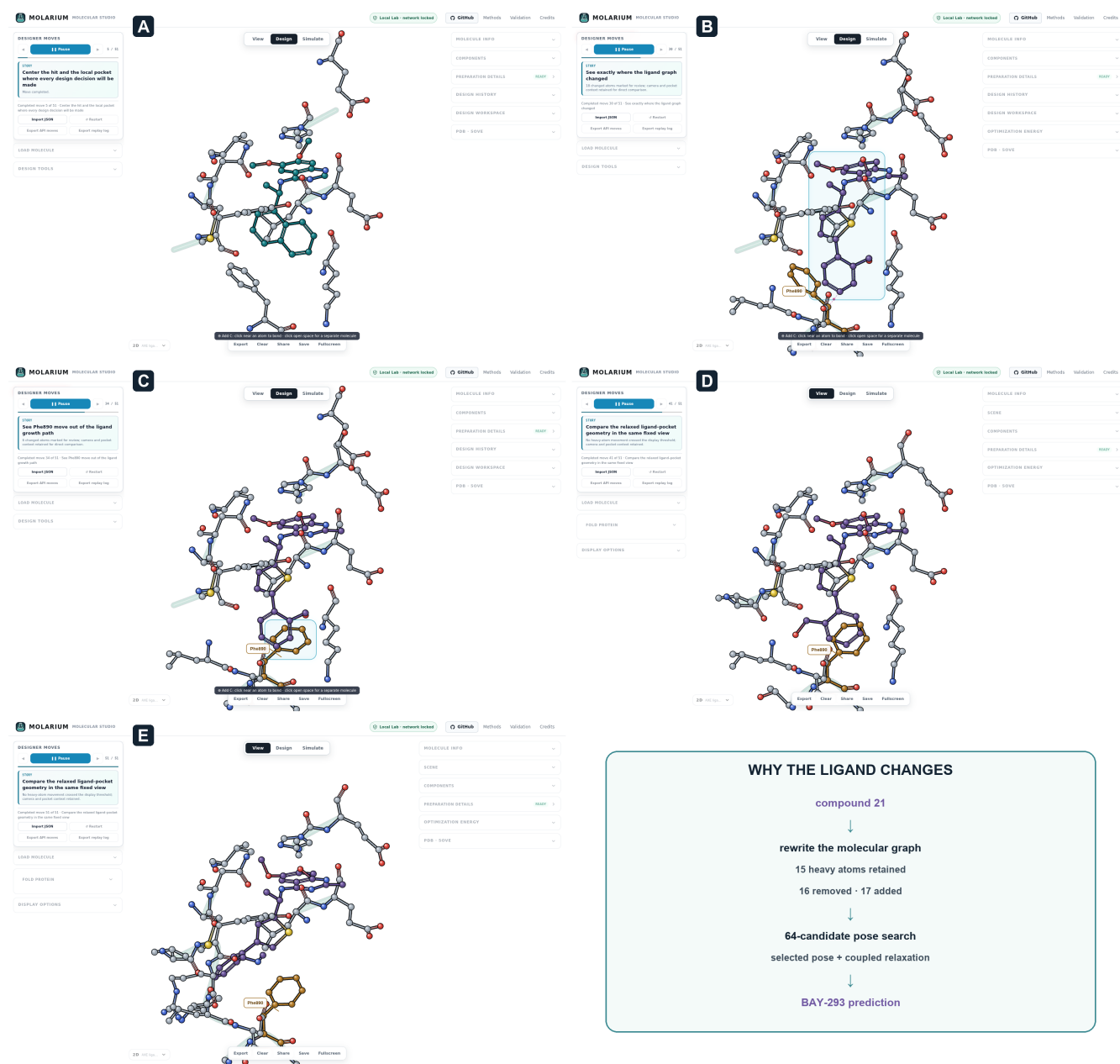
Figure 2: Hit-only SOS1 design replayed in the Molarium interface through the public Chemist Actions API. (A) The prepared 5OVE/AXE hit (teal) and its local pocket establish the camera used throughout; 5OVE/AXE was the sole coordinate-bearing input. (B) Sequential scaffold rewriting and growth produces compound 21 (purple) in the inherited Phe890-in pocket. The cyan halo identifies the edited ligand region, gold identifies Phe890, and magenta dotted connectors mark severe ligand-protein short contacts recalculated from the live coordinates. (C) A discrete side-chain search presents alternatives and the designer chooses the Phe890-out hypothesis; only the six moved Phe890 heavy atoms are haloed. (D) In the opened pocket, a new 64-chain restrained search re-fits compound 21, applies the selected feasible pose, and couples it to the receptor during WebGPU relaxation. The ligand displacement from B to D is a modeled coordinate change produced by pose search and relaxation, not camera motion or an MD trajectory. (E) The ligand graph is rewritten from compound 21 to BAY-293, then pose-refined, selected, parameterized, and relaxed in the same fixed view. The replay ends at this prediction and never opens 5OVI. Independent post-freeze comparison with 5OVI subsequently gave a receptor-aligned, graph-symmetry-minimized ligand RMSD of 1.215 Å and Phe890 \chi_1 values of -172.43^\circ in the prediction and -166.55^\circ in the crystal; those validation coordinates did not seed the replay.
