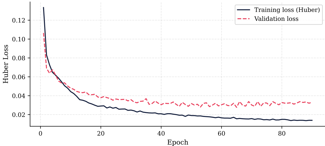
Fig. 1 — BiLSTM Training and Validation Loss
