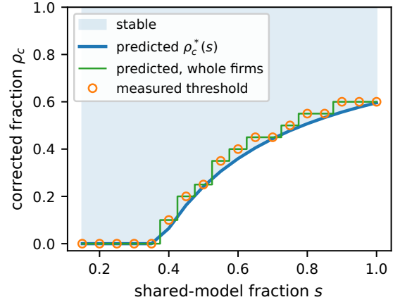
Fig. 3. Dry run: the corrected fraction needed for stability against shared-model fraction s , at N = 20 , m_1 = 0.15 , \kappa = 0.8 and near-perfect correction. Predicted and realized thresholds agree in whole firms at 18 of 18 points. Everything above the curve is stable.
