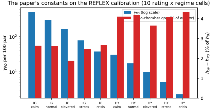
Figure 6: Real-data calibration (Table 1, calibration row). The curvature \gamma_{\text{PO}} (log scale, left axis) and the echo-chamber gap h_{\text{SP}} - h_{\text{PO}} as a percentage of the anchor (right axis) across the ten rating-by-regime cells of the REFLEX corporate-bond calibration [Nagarajan and Ashok, 2026] (IG: investment grade; HY: high yield). All ten cells reproduce within 0.8 percent.
