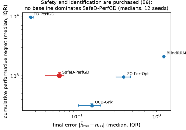
Figure 5: Baseline comparison (E6). Median final error |\bar{h}_{\text{tail}} - h_{\text{PO}}| against median cumulative performative regret over 12 seeds (bars: interquartile range) for the certified agent (SafeD-PerfGD) and four baselines. No baseline dominates it: FD-PerfGD attains lower error at roughly ten times the regret, and UCB-Grid lower regret at higher error. Safety and identification are purchased, not free.
