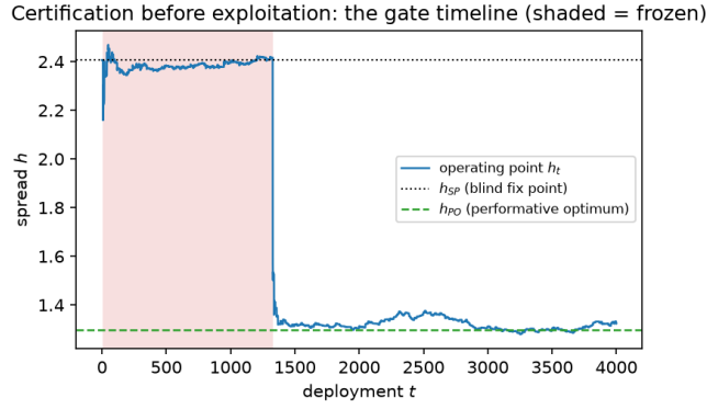
Figure 4: Certification before exploitation (L4, P7.1). Operating point h_t of the certified agent over 4,000 deployments. In the shaded interval the confidence sequence cannot yet certify that correcting is safe, so the agent stays frozen near the blind fixed point h_{SP} ; once certified, it moves to the performative optimum h_{PO} and remains inside the trust region (Table 1: 0 violations).
