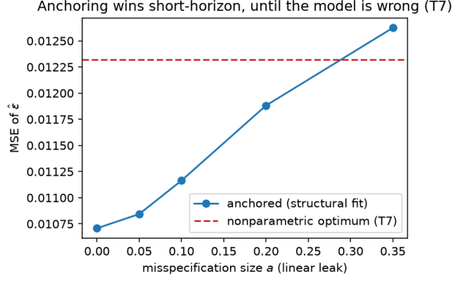
Figure 3: Anchoring crossover (T7). Mean squared error of the anchored structural fit against the size a of a linear misspecification the family cannot represent, compared with the budget-and-horizon-optimal nonparametric estimator (dashed). Anchoring wins at small misspecification and loses past the crossover near a \approx 0.29 , as T7 predicts. Pivot E5 replaced an exponential misspecification, which had decayed to about 10^{-3} by the operating point and was correctly invisible to the fit, with this linear leak.
