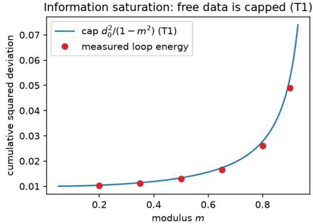
Figure 2: Information saturation (T1). Cumulative squared deviation of the noiseless retraining trajectory against the modulus m ; the cap d_0^2/(1 - m^2) (line) matches the measured loop energy (points). Without deliberate exploration, the information a retraining loop reveals about its own performativity is bounded, and the bound grows with m . Pivot E1 added to this picture the excitation floor (\sigma/\gamma)^2/(1 - m^2) that noisy observations contribute (Table 1, feedback-floor row).
