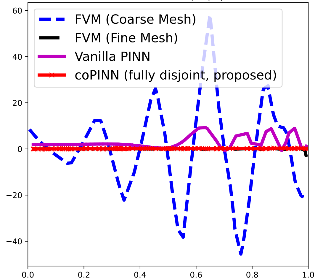
Residuals f_1(x)
