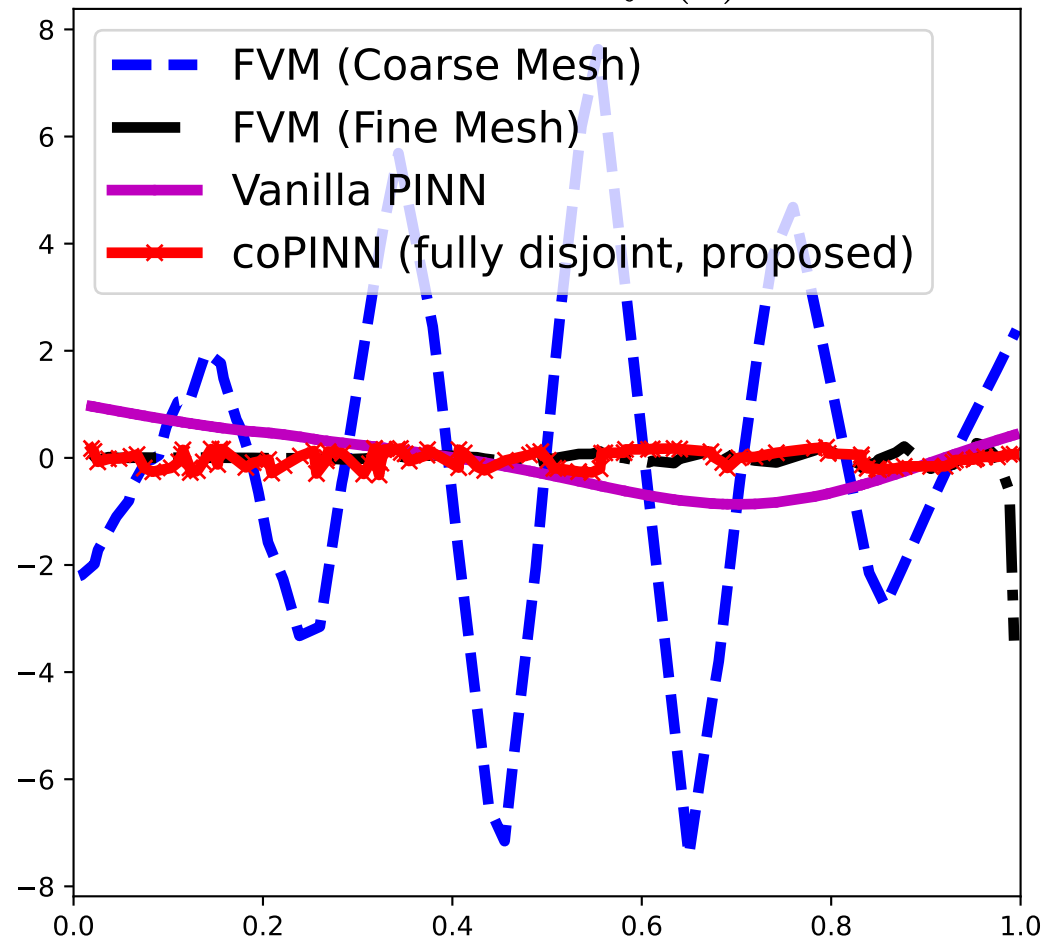
Residuals f_2(x)
